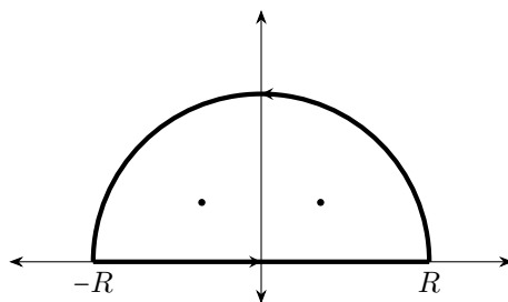
Figure 4: Contour in the upper half-plane, with the two points denoting the two simple poles of f(z) in the upper half-plane.
